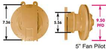
Typical Fan Clutch - Ford w/ Cummins NTC
