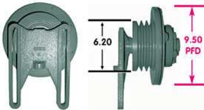
Typical Fan Clutch - Kenworth w/ Cummins
