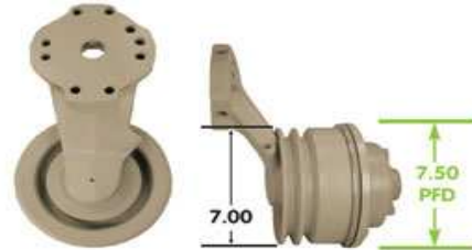
Typical Fan Clutch - Ford w/ Cummins NTC
