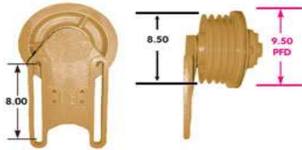
Typical Fan Clutch - Kenworth w/ Cummins
