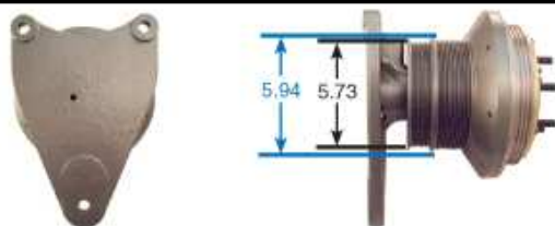
Typical Fan Clutch - Mack Applications
