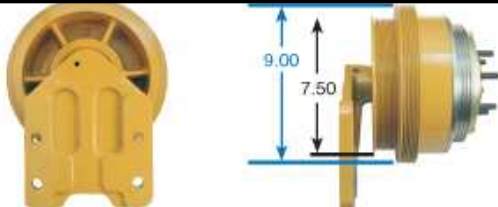
Typical Fan Clutch - Peterbilt w/ 3406 Cat.
